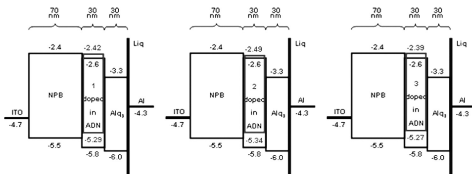
Figure 2. Relative energy-level alignments and layer thickness of OLEDs.
