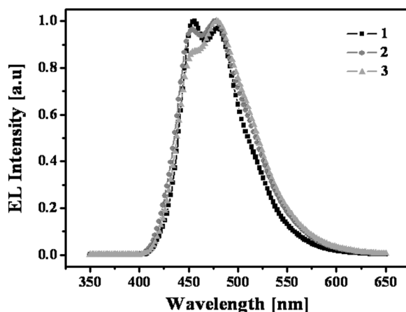
Figure 3. Electroluminescence spectra of devices 1–3.
