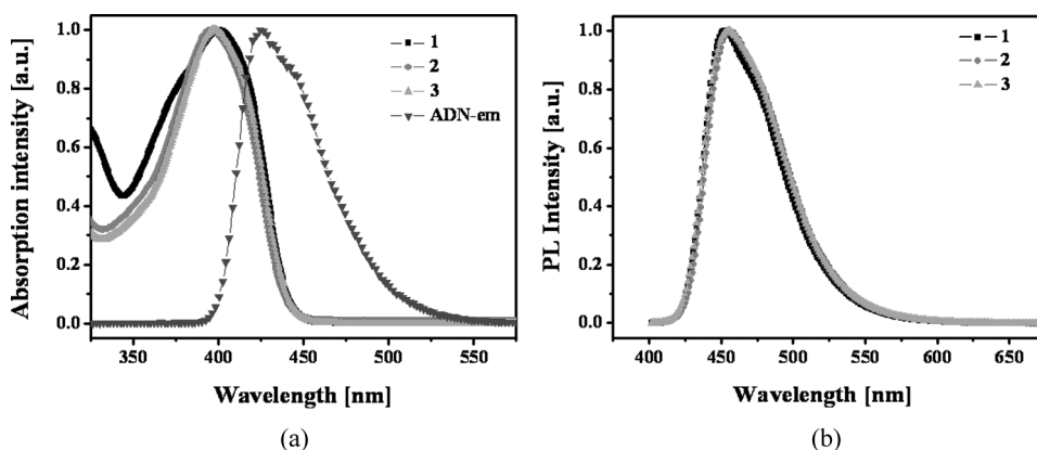
Figure 1. (a) UV-vis absorption and (b) photoluminescence spectra of compounds 1–3 in a 10^{-5} M dichloromethane solution.
