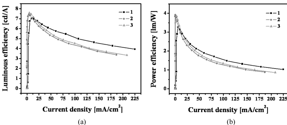
Figure 5. (a) Luminous efficiencies and (b) power efficiencies as a function of current density for the devices 1–3.
